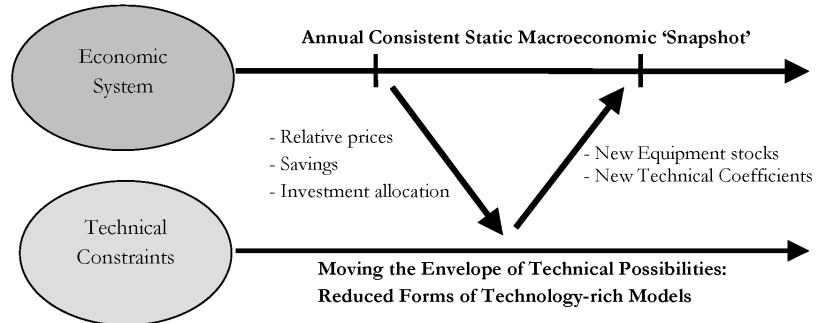
Figure 1 Iterative top-down/bottom-up dialogue in IMACLIM-R
