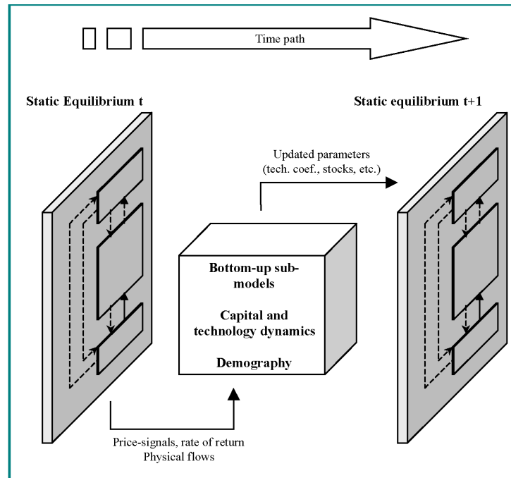
Figure 2 The recursive dynamic framework of IMACLIM-R (see online version for colours)
